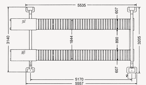
UPPER LIFT FOR WHEEL-FREE (FP3500X and FP4000X)
